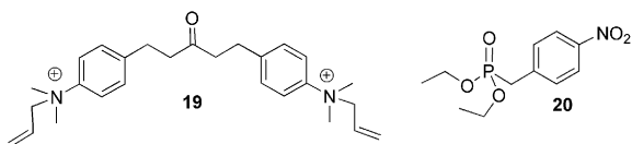
Fig. 15 Chemical structure of the simulants 19 and 20 .
